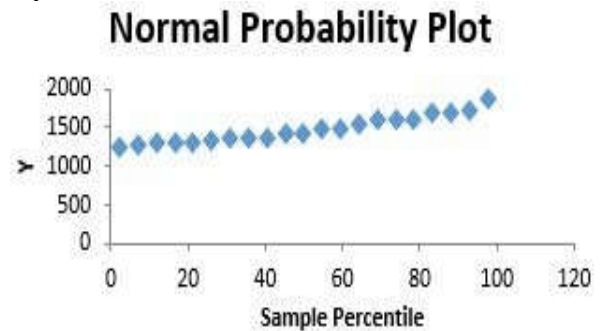
Gambar 1. Grafik normal probability plot
