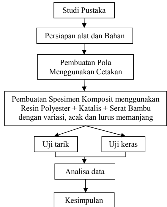
Gambar 5. Diagram Alir
