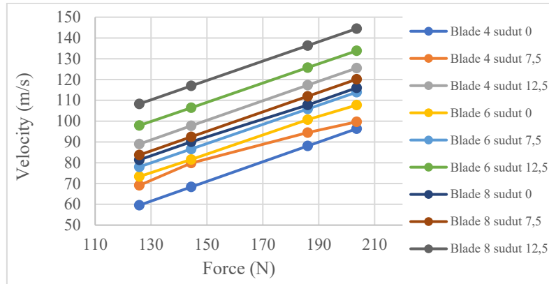
Gambar 7. Nilai Force Terhadap Velocity.
