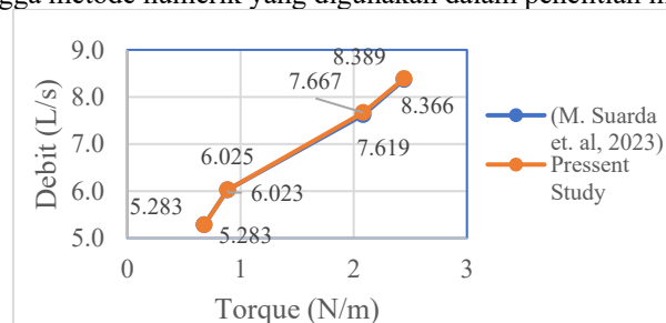
Gambar 6. Nilai Torque Terhadap Debit.
