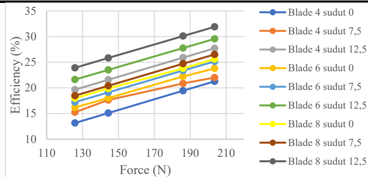
Gambar 12. Nilai Force Terhadap Efficiency.
